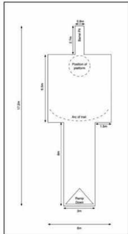
Improved 105 Gun Pit
